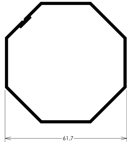
MN015 0,881 kg/m Tubo octogonal 60 integrada
