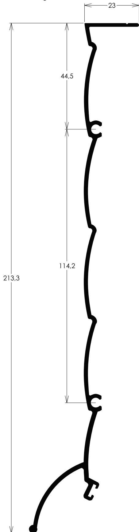
MN039 1,400 kg/m Tampa externa integrada
